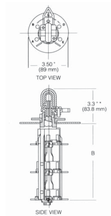
Figure 8. Two and Three-Phase Cap/Wrench Operable Switch.
