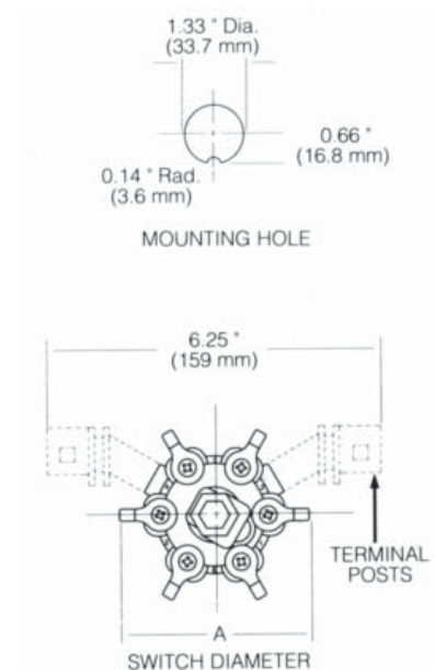
Figure 7. One-Phase Mounting Hole and Switch with and without Terminal Posts.
