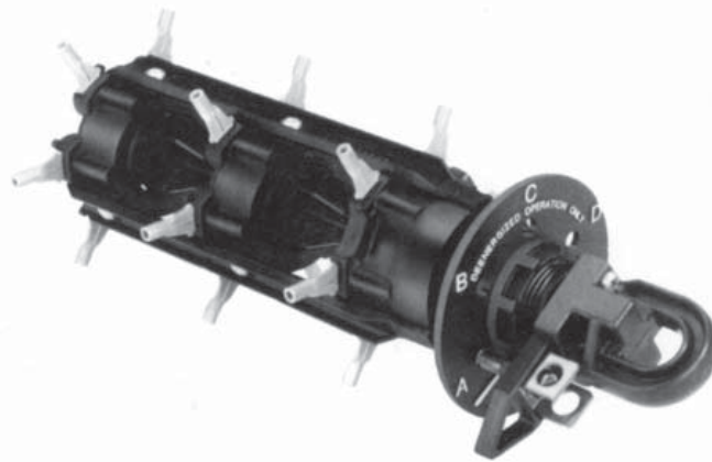
Figure 2. Three-Phase Tap Changer with Padlockable Flexible Hookstick Pointer Handle and Index Plate..
