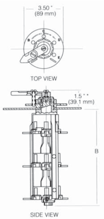
Figure 10. Two and Three-Phase Lever Handle Switch.
