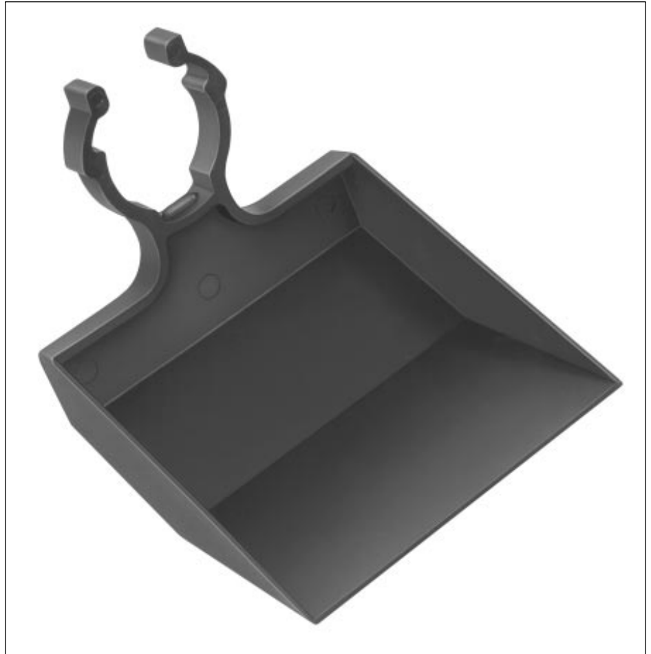
Figure 1. Drip Guard for sidewall mount Bay-O-Net fuse assembly.
