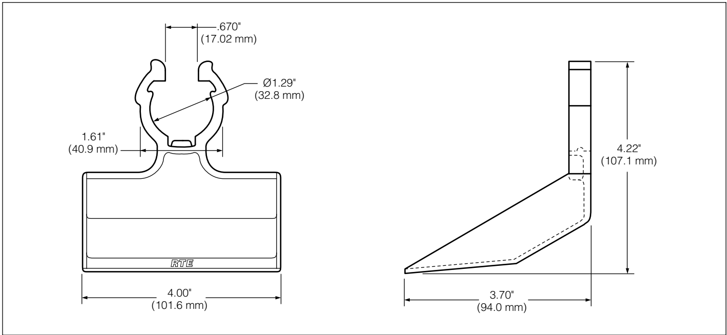
Figure 2. Dimensional information for front and side views.
